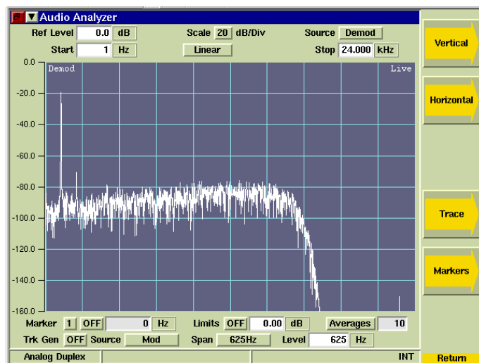
Figure 6. Audio Analyzer
